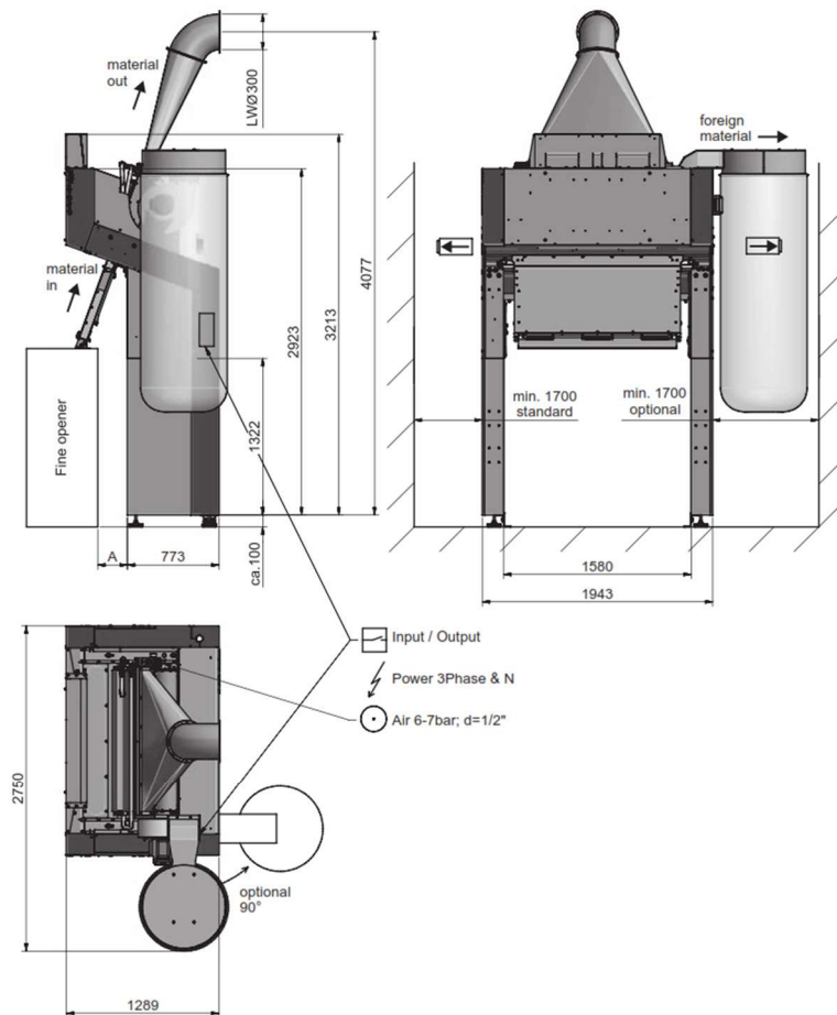
Technical drawing USTER® JOSSI VISION SHIELD 2
